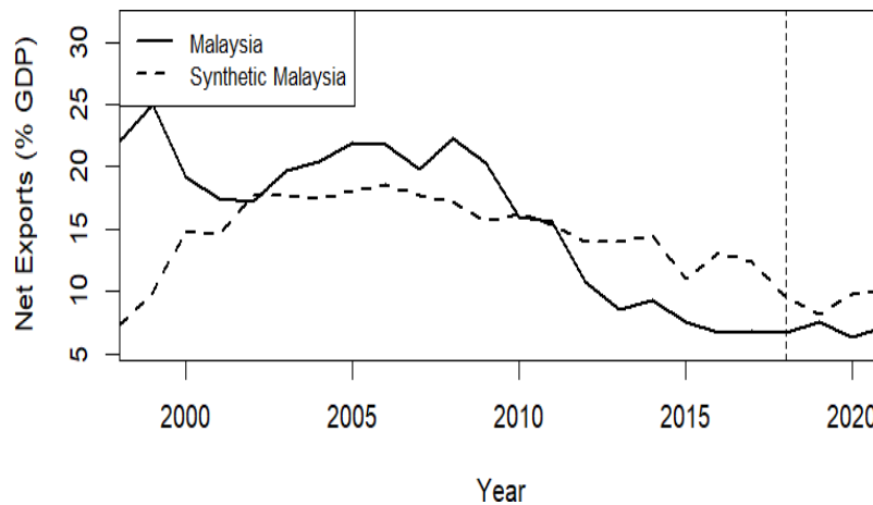
Figure 5: GDP component (net exports) of Malaysia against synthetic Malaysia
